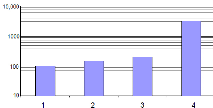
Figure 2-10: Relative mean threshold and discomfort stimulation levels
