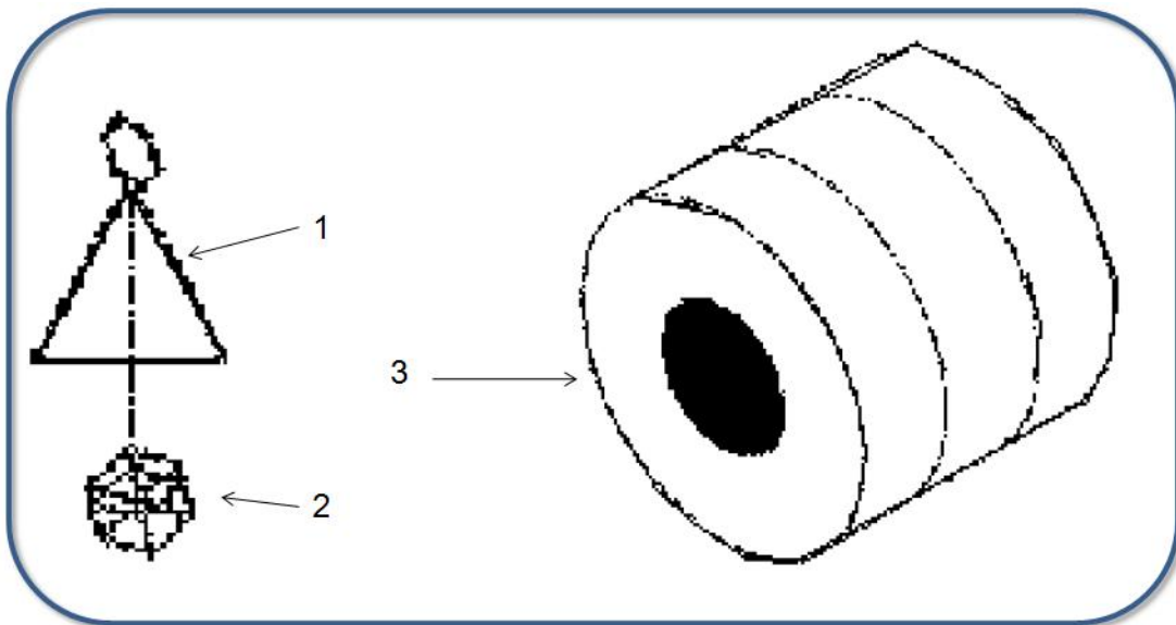
Figure 2-43: 1 = deflection meter, 2 = mesh bag, 3 = magnet
