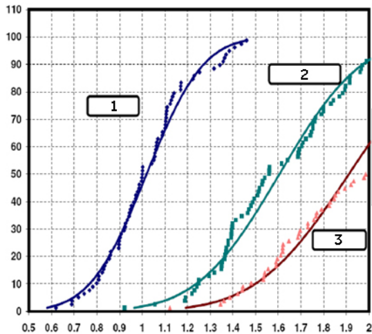
Figure 2-11: PNS probability. X axis = Fraction of the Mean Threshold (100% PNS). Y axis = Population percentile.
